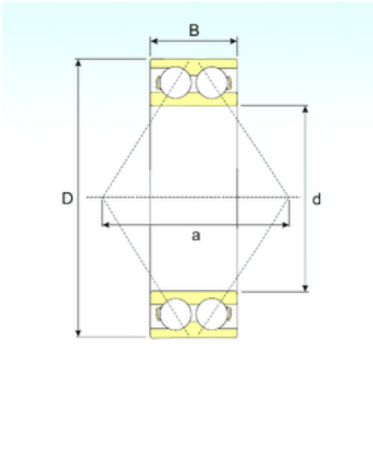
3308 Bearing 2D drawings and 3D CAD models
